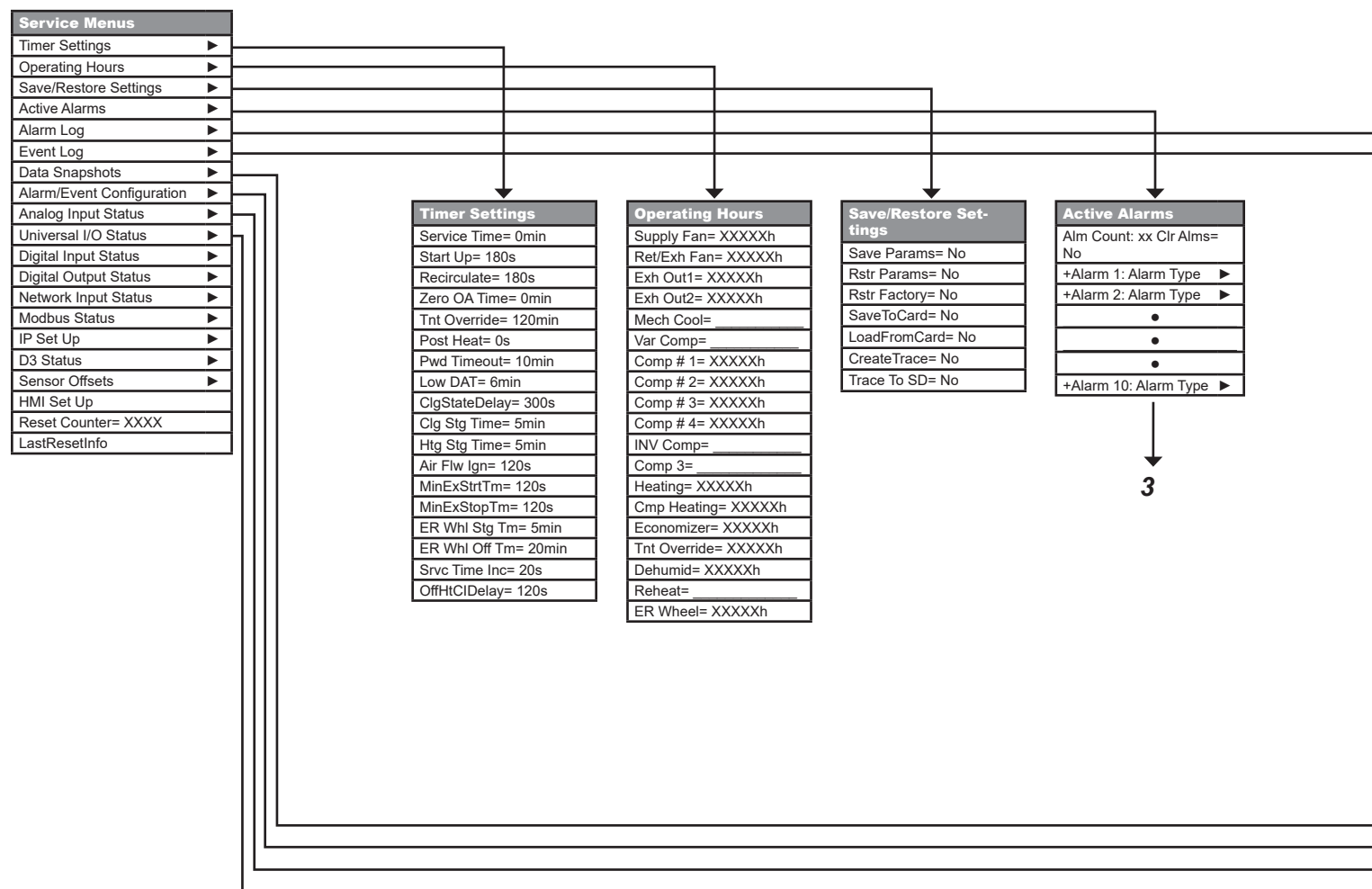
Figure 7: Service Menu – Keypad/Display Menu Structure
