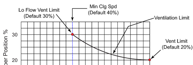
Figure 13: Damper Position versus Fan Speed Chart
