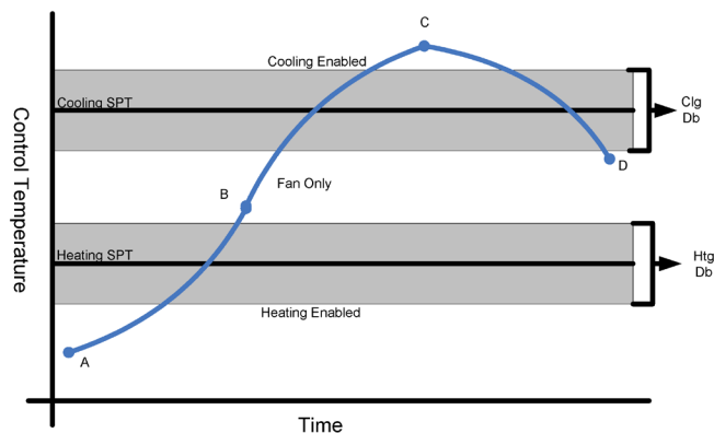
Figure 11: Heat/Cool Changeover
