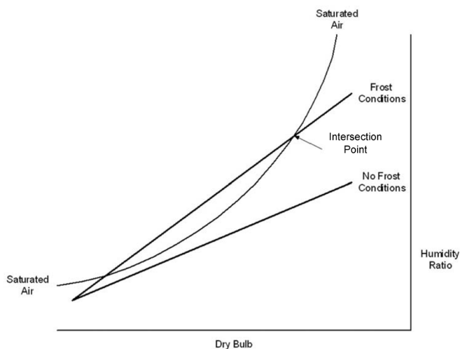
Figure 12: Exhaust Air Psychometric Chart
