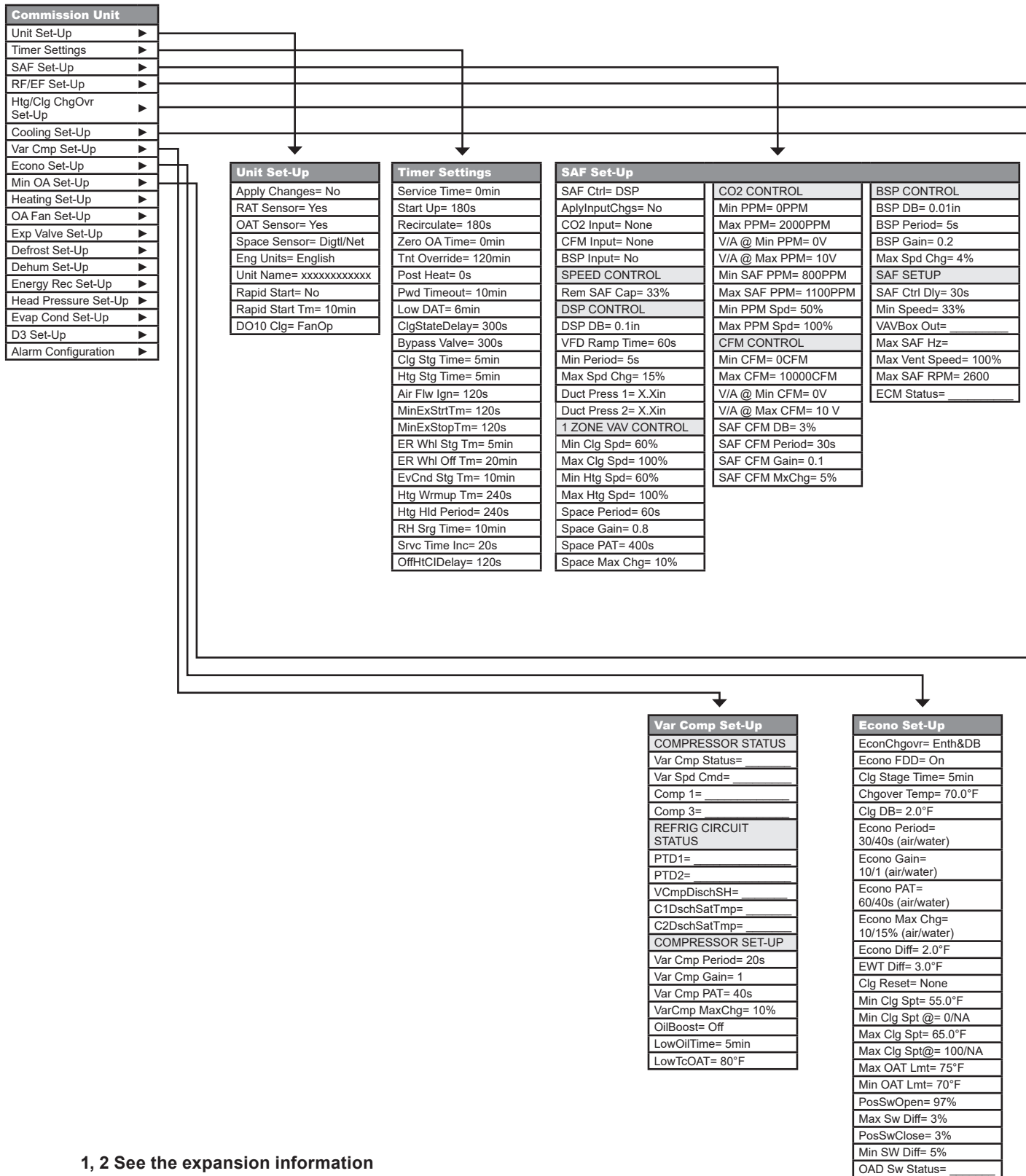
Figure 6: Commission Unit – Keypad/Display Menu Structure
